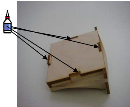
12. Apply glue to notches in drawer bottom and assemble to drawer.
