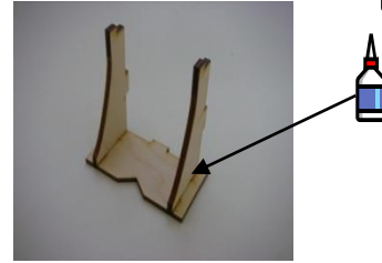
9. Glue and assemble the other drawer side the same way.
