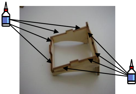
11. Place drawer upside down and apply glue to all notches.
